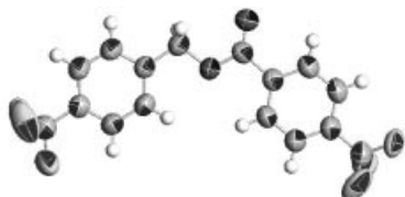
Figure 1. ORTEP plot of p -(trifluoromethyl)benzyl p -(trifluoromethyl)benzoate ( 21 ) at 50% probability
